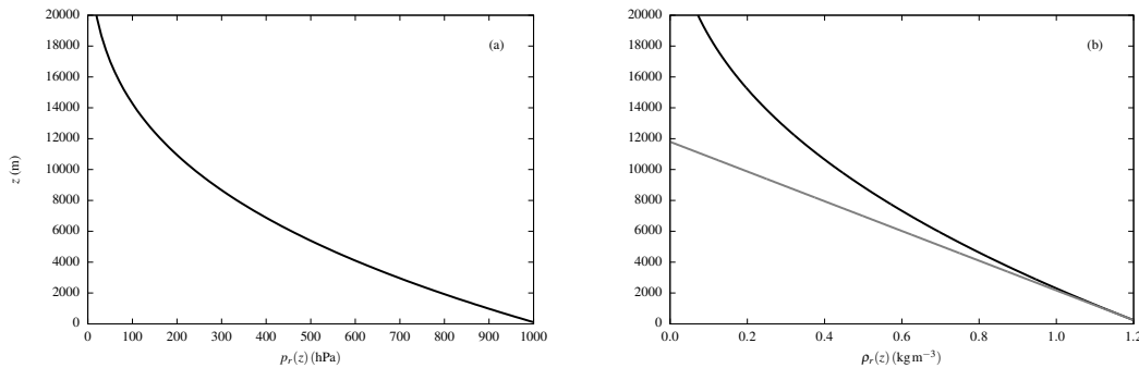
Figure 3.1: Reference pressure p_r and density \rho_r in a hydrostatic and adiabatic equation.
